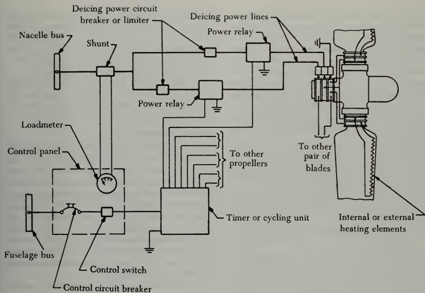
FIGURE 7-26. Typical electrical deicing system.
